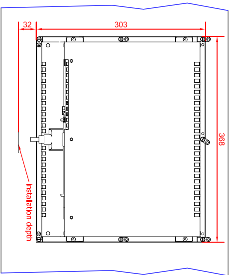
rear view with install measure
