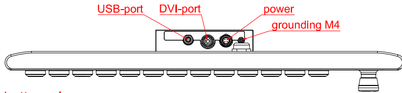
bottom view
