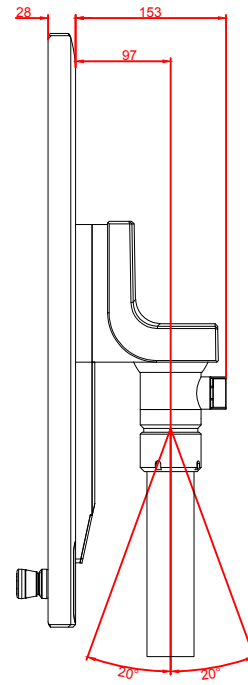
right view
