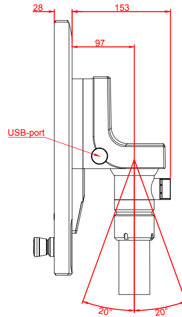
right view
