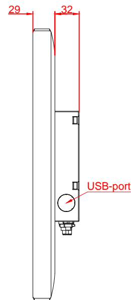
left view
