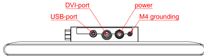
bottom view
