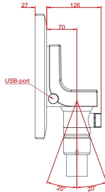
right view
