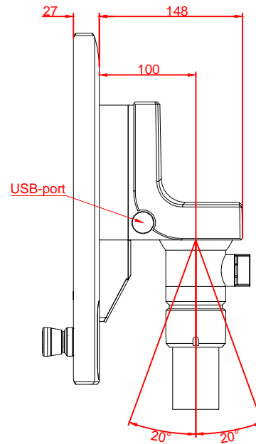
left view
