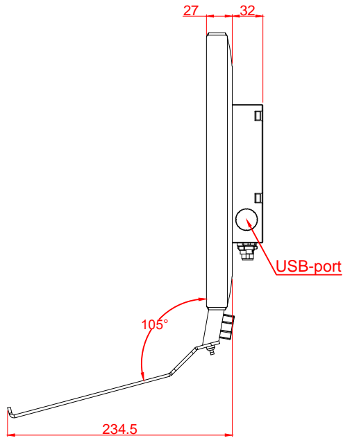
left view
