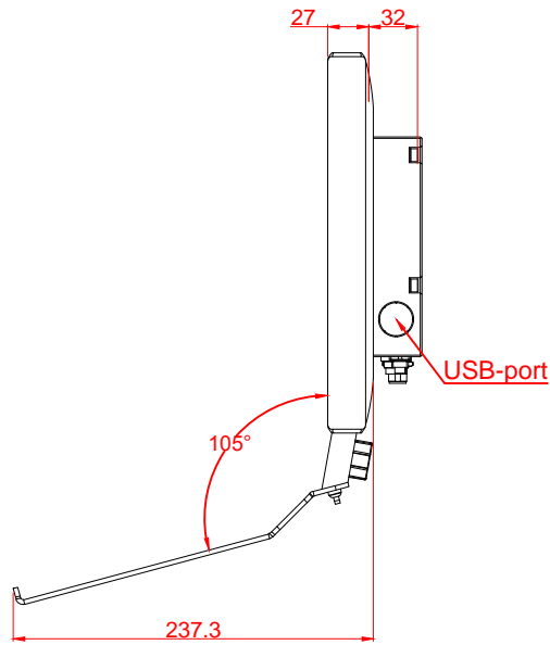
left view
