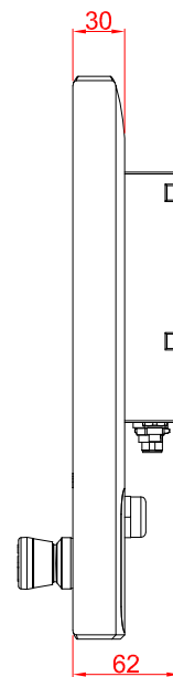
right view
