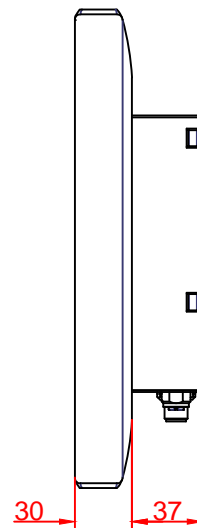
left view
