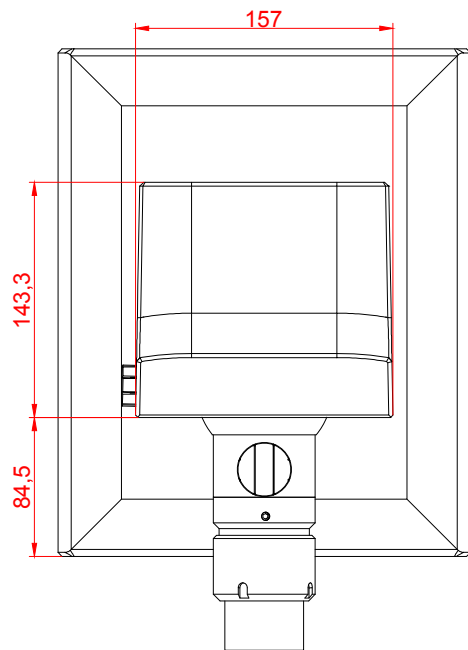
rear view
