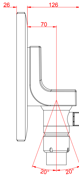
right view
