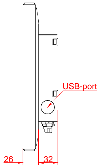
right view
