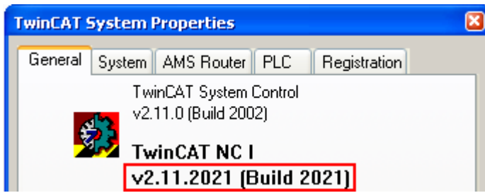
Fig. 83: TwinCAT Version
