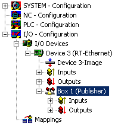
Fig. 61: Insert a Publisher Box
