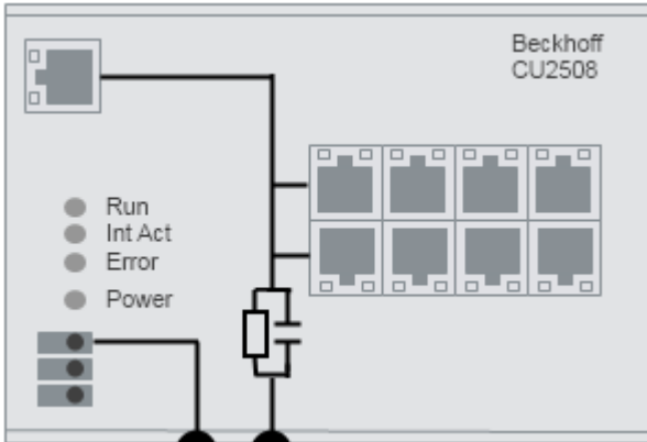
Fig. 22: CU2508 shield concept
