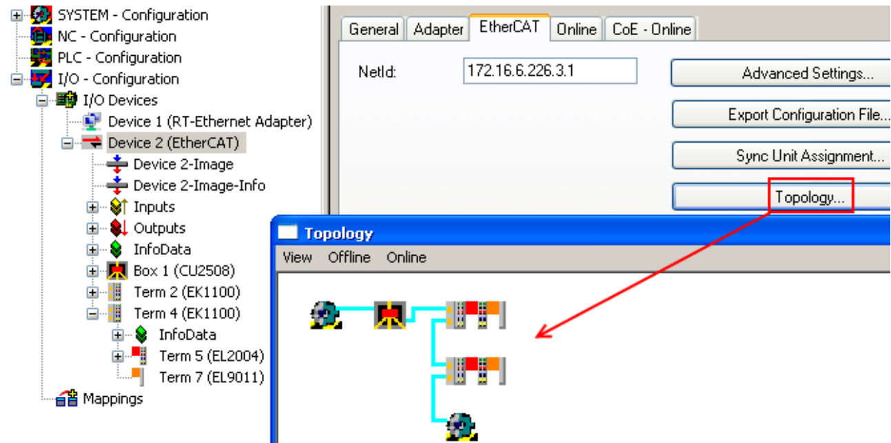
Fig. 45: Checking topology with EtherCAT cable redundancy
