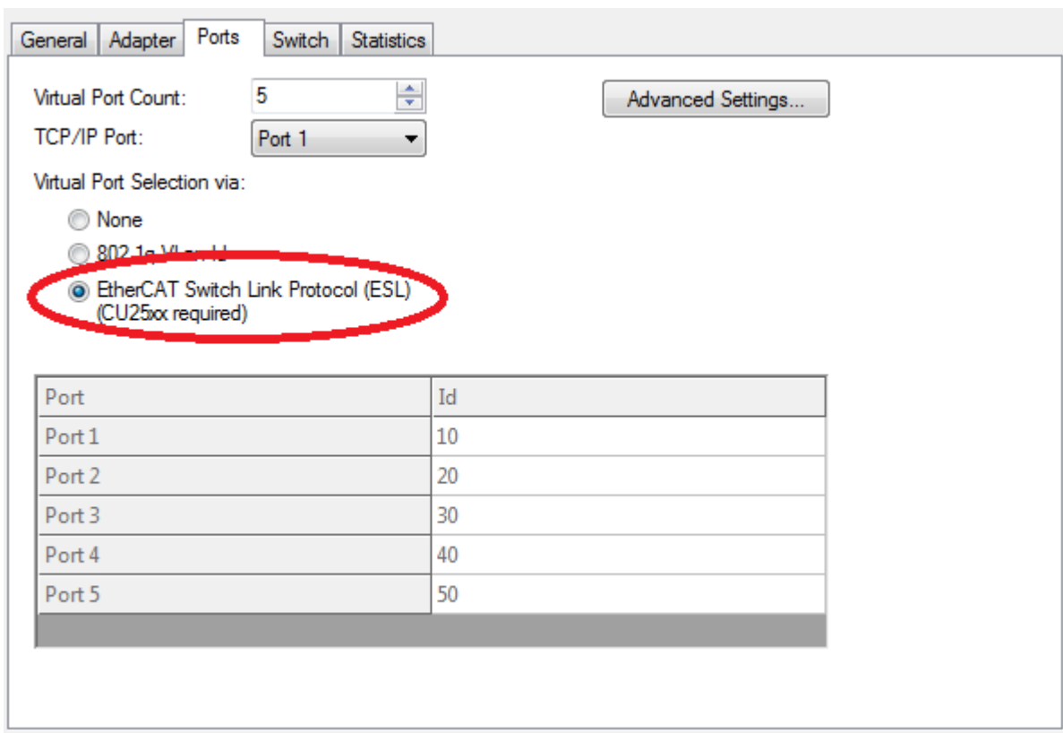
Fig. 58: Selection of the "Virtual Port" setting
