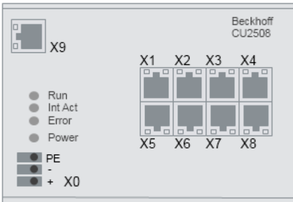
Fig. 21: CU2508 front view
