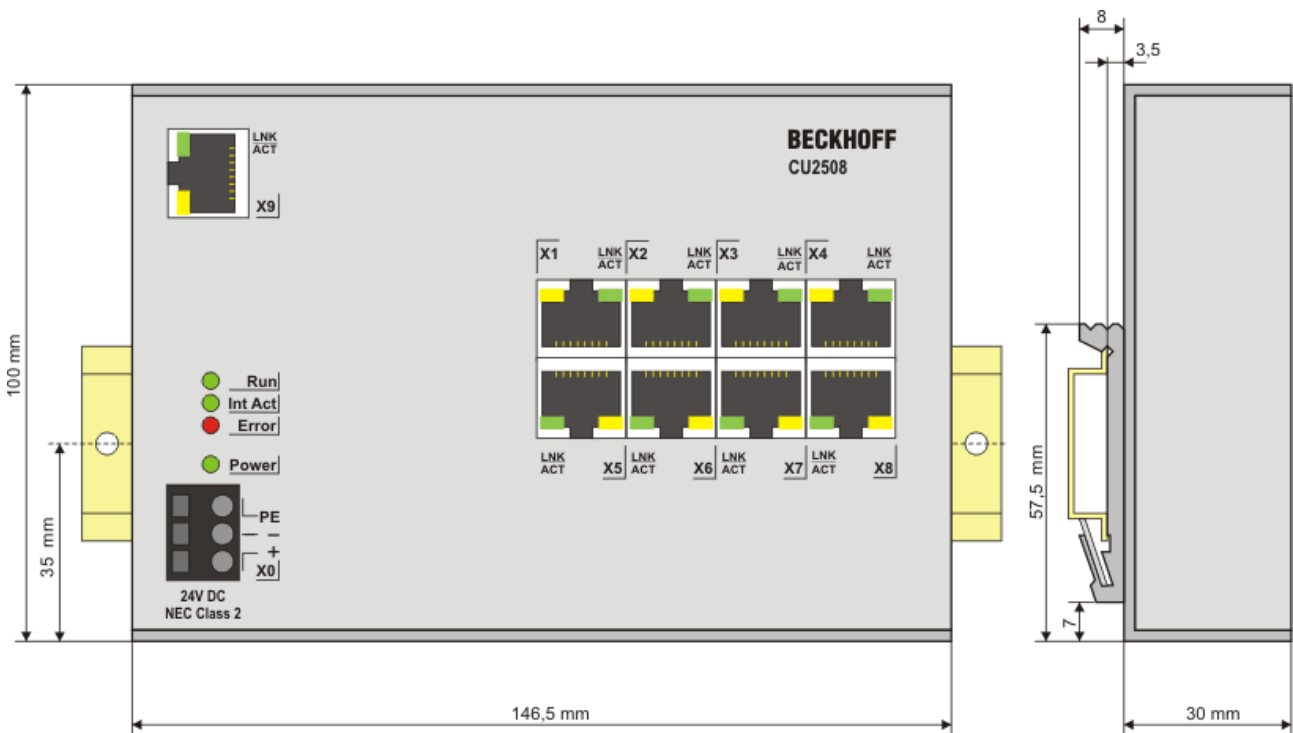
Fig. 14: CU2508 dimensions
