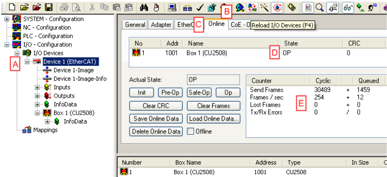
Fig. 90: Online configuration
