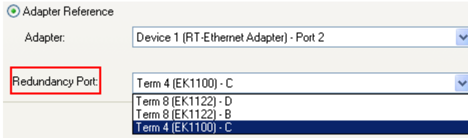
Fig. 44: Specification of the field-side redundancy port
