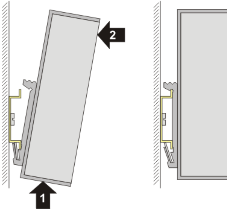
Fig. 17: Mounting
