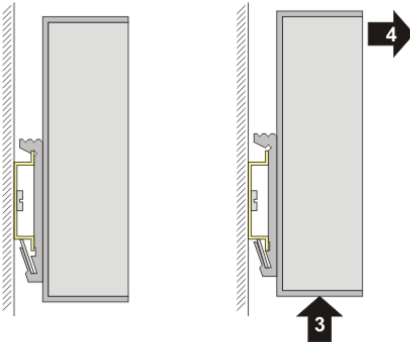
Fig. 18: Removal
