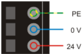
Fig. 19: CU20xx – Supply connector
