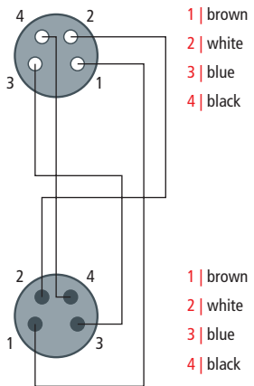
Plug, 4-pin
