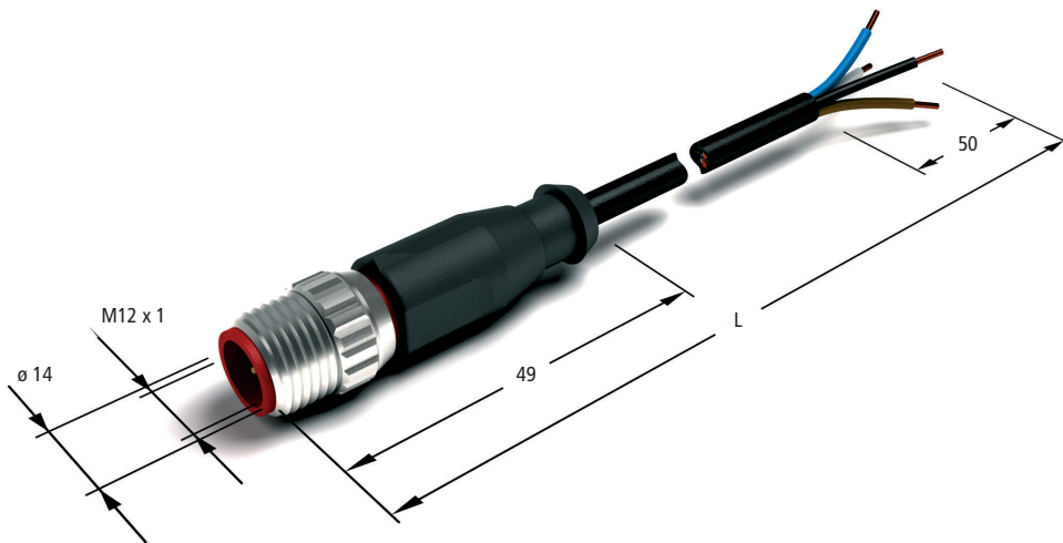
Plug, 4-pin
