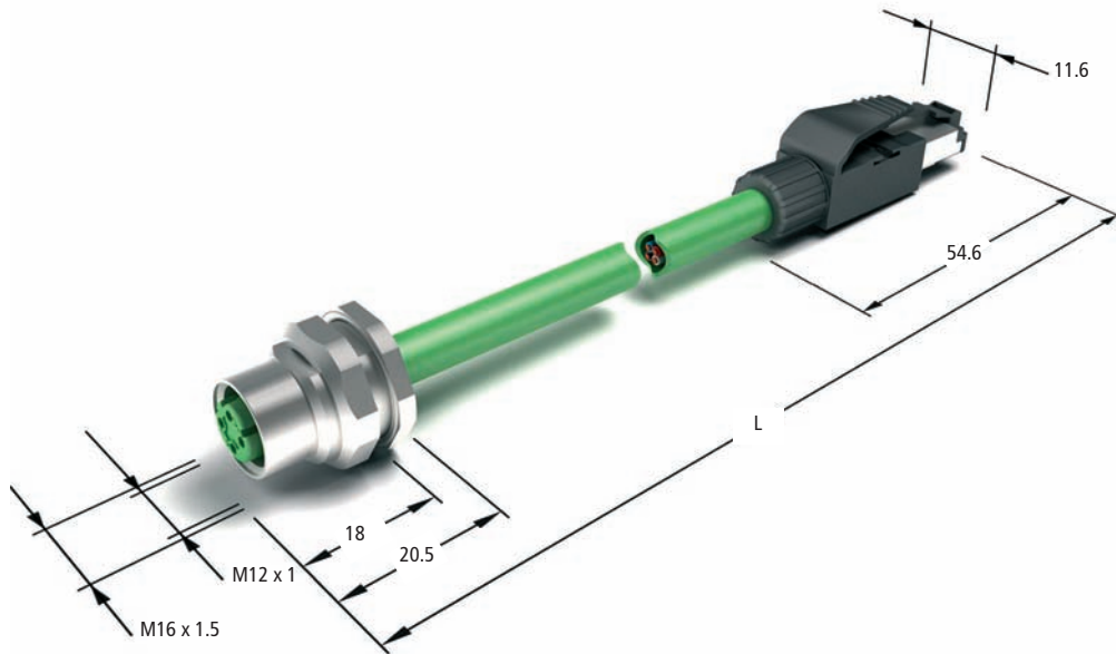
RJ45, 8-pin
