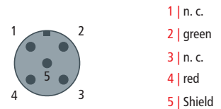
Plug M12, 5-pin
