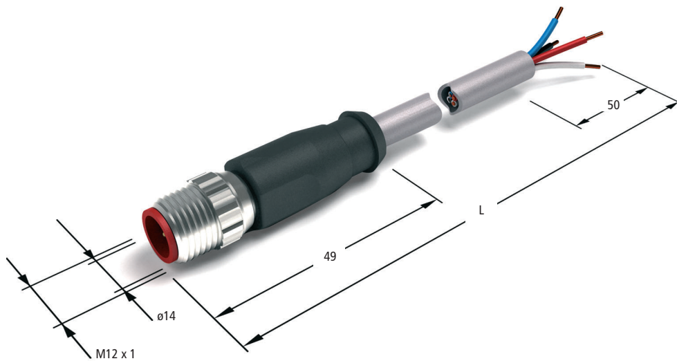
Plug M12, 5-pin
