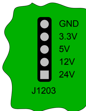
Figure 3 Pinout of the header J1203
