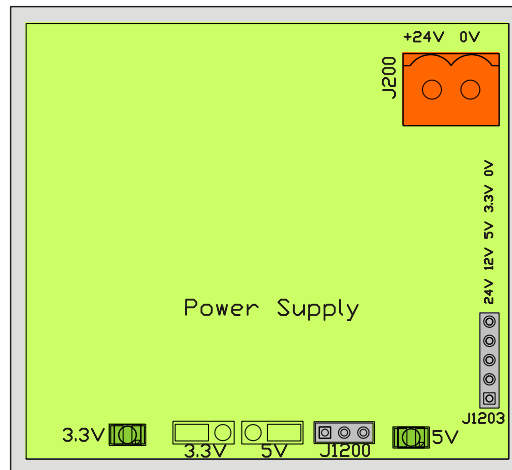
Figure 2 Power Supply
