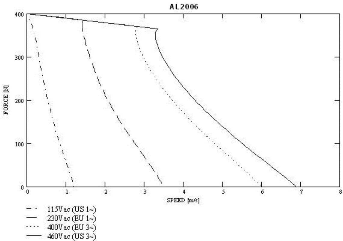
Velocity diagram AL2006
